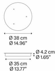
Ceiling Canopy
