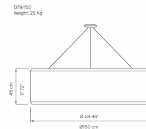
D79/150 weight: 29 Kg
