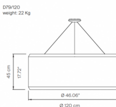
D79/120 weight: 22 Kg
